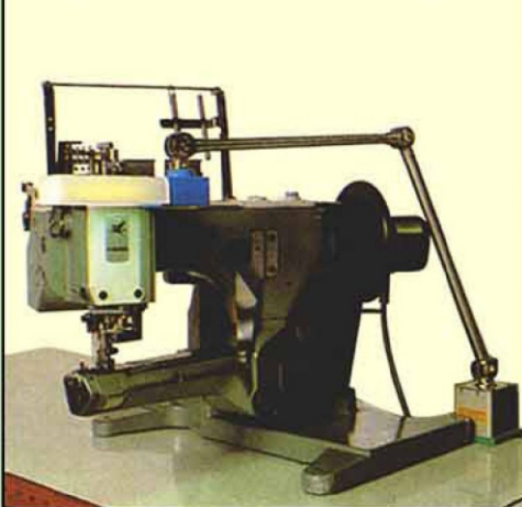
DS-27K M-BRACKET
